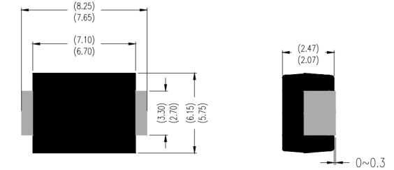
SMC/DO-214AB
